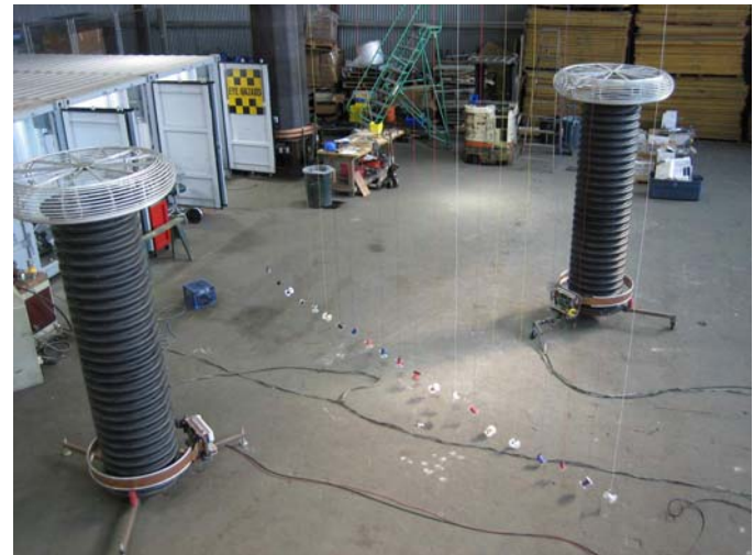
Fig. 5. Electrostatic test curtain in position between transformers.
